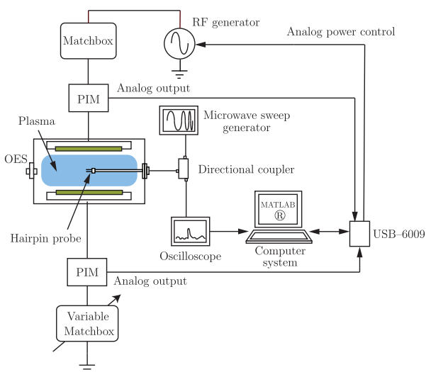
Figure 3: Experimental apparatus for real-time VM and control of electron density and plasma etch rate.
