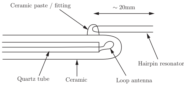
Figure 4: Microwave resonator hairpin probe.
