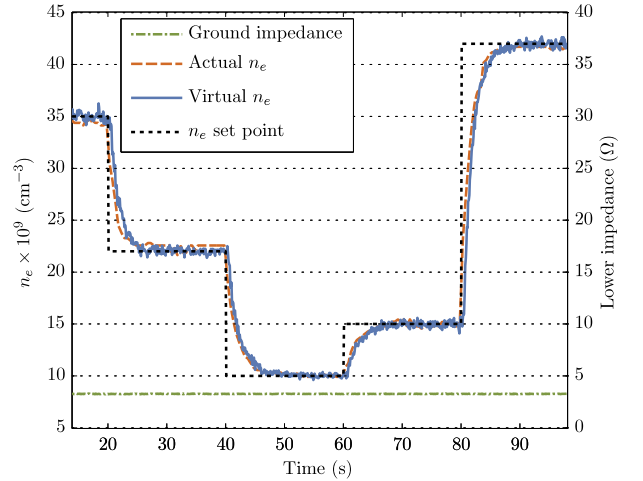
Figure 8: PFC control of electron density with T_s = 0.1 s, \tau_r = 1 s, at constant pressure and with no disturbances to the ground impedance.
