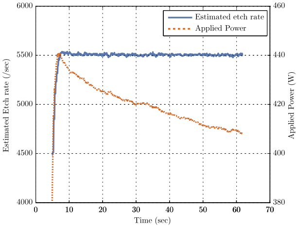
Figure 11: Startup transients with PFC control. The initial startup irregularities shown in Figure 10 are much less pronounced because the PFC controller explicitly deals with the system delay in the VM system.
