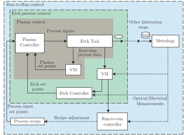
Figure 2: Virtual metrology and control implementations for plasma etch [4].
