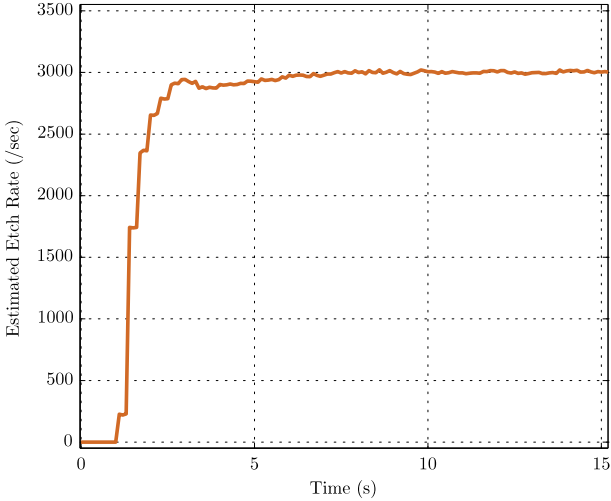
Figure 11: Startup transients with PFC control. The initial startup irregularities shown in Figure 10 are much less pronounced because the PFC controller explicitly deals with the system delay in the VM system.
