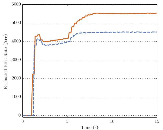
Figure 10: Startup transients with PI control. Undesirable irregularities are observed as the plasma ignites due to pressure changes in the chamber.
