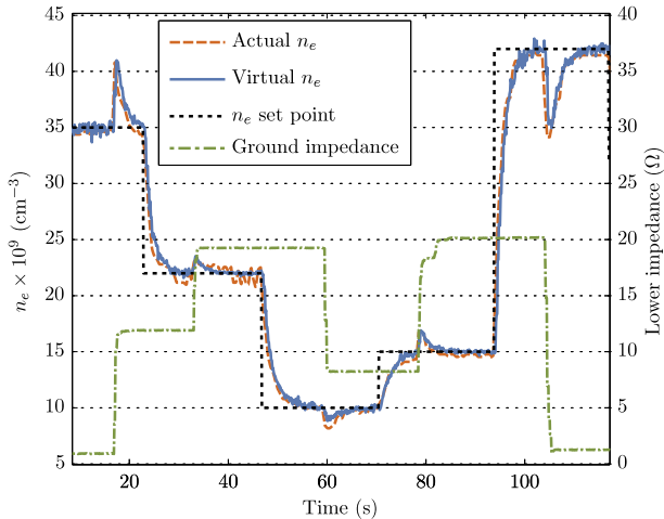
Figure 9: PFC control of electron density with T_s = 0.1 s, \tau_r = 1 s, at a constant pressure in the presence of unmeasured disturbances in ground impedance.
