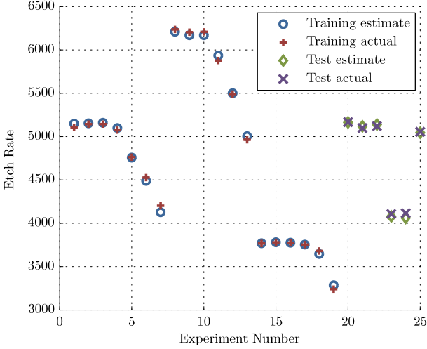
Figure 6: Etch rate estimates from linear regression model.
