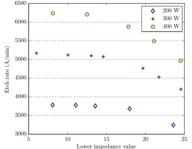
Figure 5: Average etch rate achieved during data collection for VM modelling.
