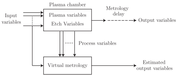
Figure 1: Virtual metrology principle. Estimates of process output variables of interest are made using process variables and mathematical models, or virtual metrology models.
