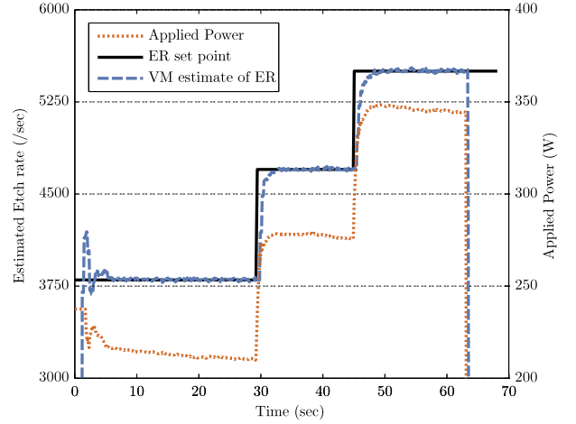
Figure 13: Estimated etch rate for wafer etch with step changes in etch rate during etching. The etch depth can be estimated with an accuracy of 0.81% by integrating the VM signal.
